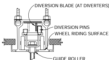
TYPE 7/8 TRACK WITH PRE-PROGRAMMED™ DIVERSION PINS
