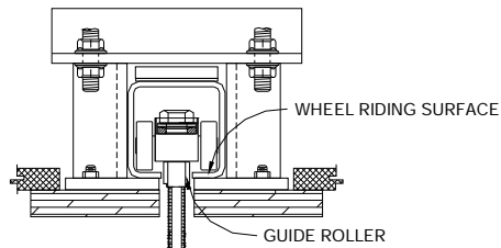
TYPE 5 TRACK
